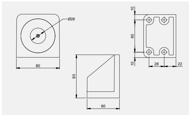
Dimensions - Strike
