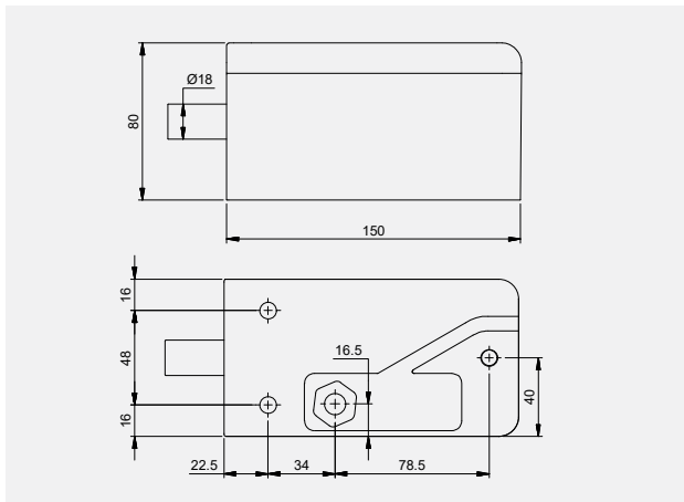
Dimensions - Lock
