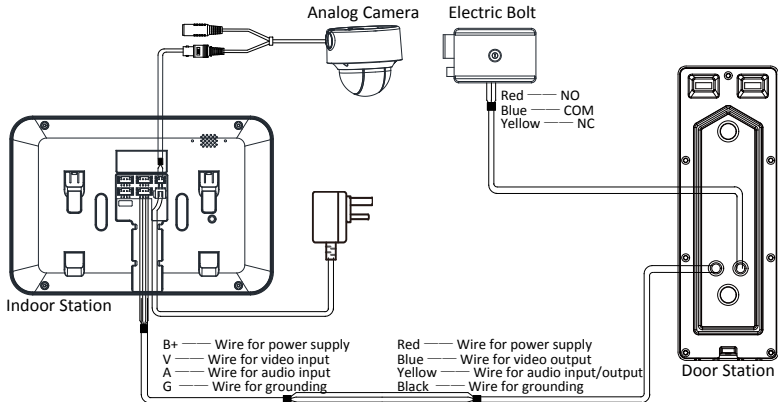
Figure 3-3 Wiring 1 (1 Door Station and 1 Indoor Station)
