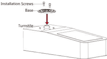
Figure 3-13 Install Base
