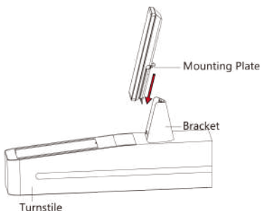
Figure 3-25 Install Device
