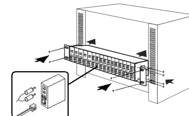
Figure 6-1 Installing Media Chassis in Wiring Closet Rails
