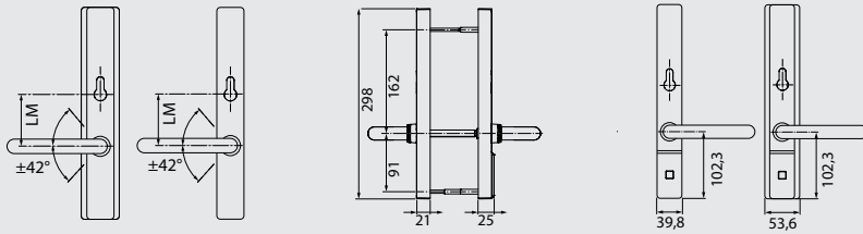
c-lever pro, standard version. Type 2621 (narrow) and 2622 (wide)
