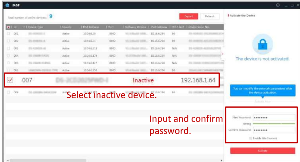
Figure 2-4 SADP Interface
