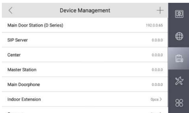
Figure 2-3 Device Management
