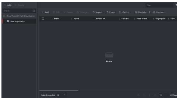
Figure 3-22 PersonalManagement Application
