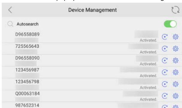
Figure 2-4 Device Information
