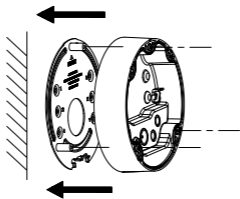
Figure 2-9 Secure the Junction Box
