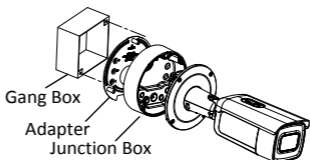
Figure 2-14 Mounting with a Gang Box
