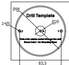
Figure 2-10 The Drill Template
