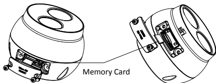
Figure 2-24 Install Memory Card
