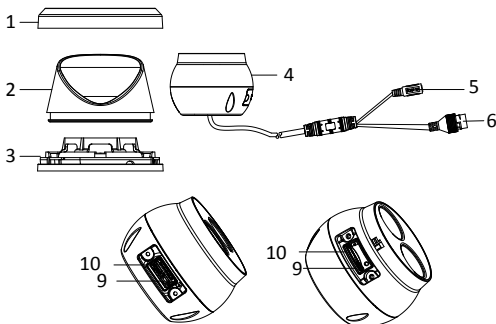
Figure 1-3 Type IV Turret Camera
