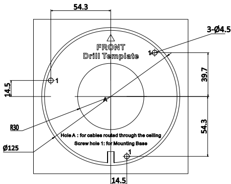
Figure 2-25 Drill Template
