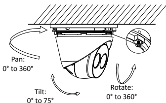
Figure 2-28 Adjust Surveillance Angle
