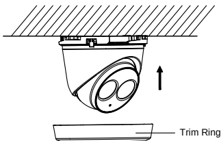
Figure 2-22 Install the Trim Ring
