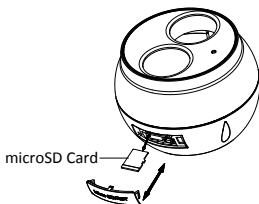
Figure 2-17 Memory Card Slot
