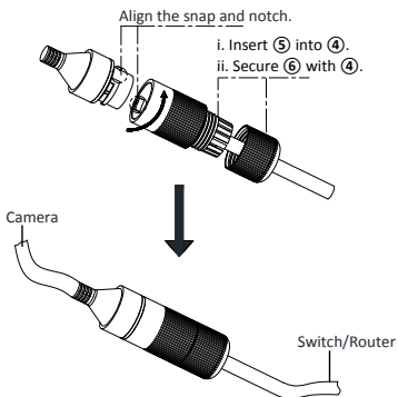
Figure 2-38 Water-proof Accessory Installation
