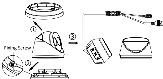
Figure 2-23 Disassemble the Camera
