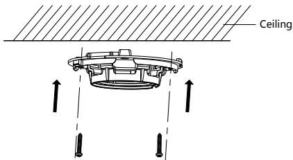
Figure 2-12 Secure the Camera to the Ceiling
