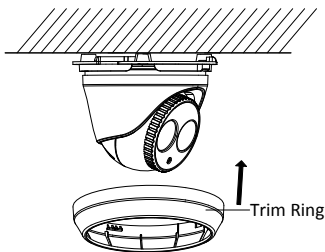
Figure 2-8 Install the Trim Ring
