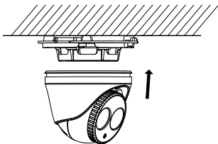
Figure 2-5 Secure the Camera to the Mounting Base
