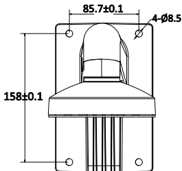
Figure 2-30 Dimension of Demonstrated Wall Mounting Bracket
