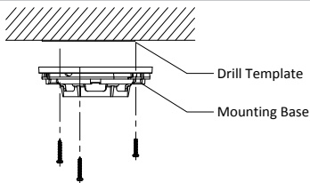
Figure 2-26 Fix Mounting Base
