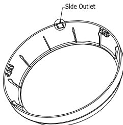
Figure 2-3 Side Outlet
