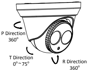
Figure 2-7 Adjust the Lens
