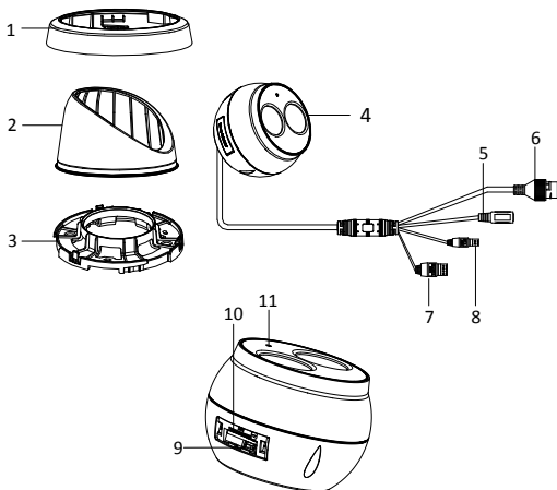
Overview of Type III Turret Camera
