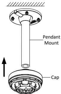
Figure 2-35 Install the Cap
