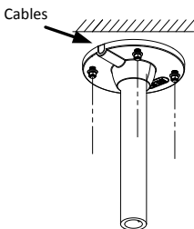
Figure 2-33 Fix Pendant Mount
