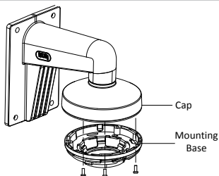
Figure 2-31 Fix Mounting Base
