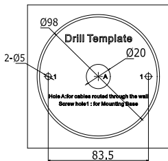
Figure 2-18 The Drill Template
