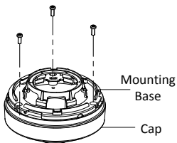
Figure 2-34 Fix Mounting Base
