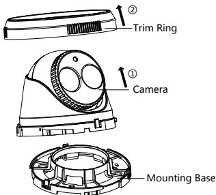
Figure 2-9 Disassemble the Camera
