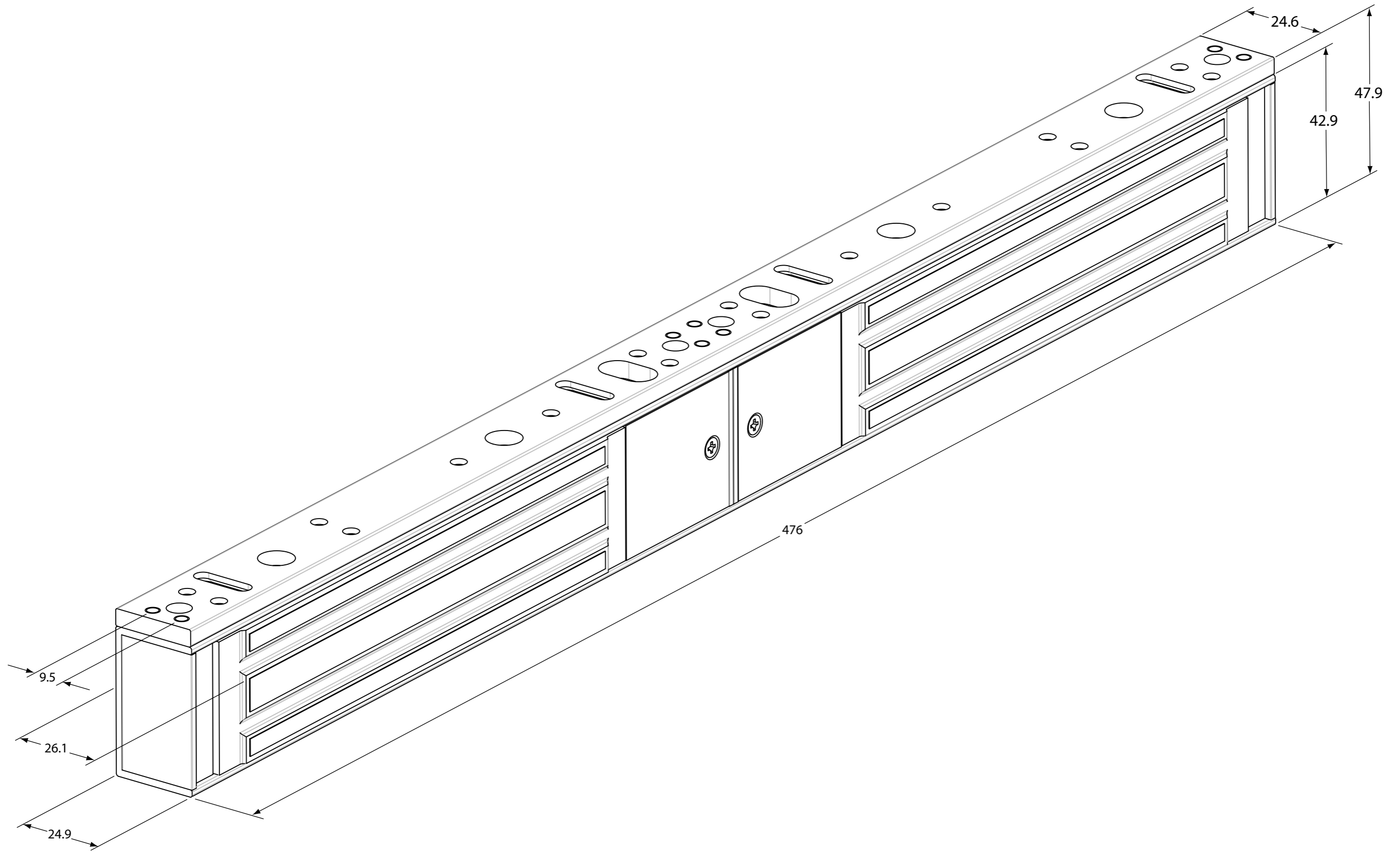
Z4 DOUBLE ELECTRO MAGNETIC LOCK ASSEMBLY
